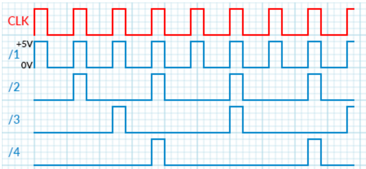
Up-beat counting for source clock (CLK 33%) and outputs from /1 to /4 (triggers).
